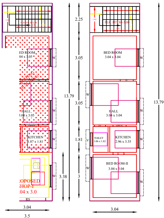
PROPOSED SHOP- 1 GROUND FLOOR PLAN SCALE 1: 100 PROPOSED FIRST FLOOR PLAN SCALE 1: 100
