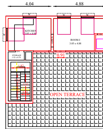
SECOUND FLOOR PLAN SCALE 1: 100
