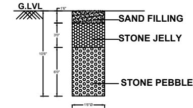
RAIN WATER HARVESTING PIT (NOT TO SCALE)
