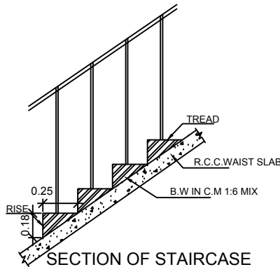
SECTION OF STAIRCASE (NOT TO SCALE)
