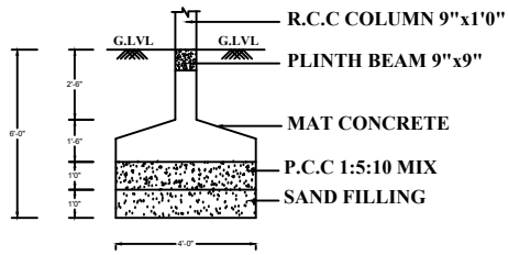
COLUMN FOUNDATION (NOT TO SCALE)
