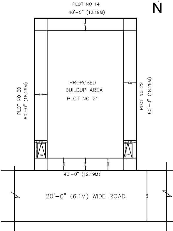
SITE PLAN
