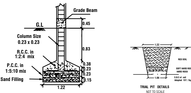
COLUMN DETAILS NOT TO SCALE
