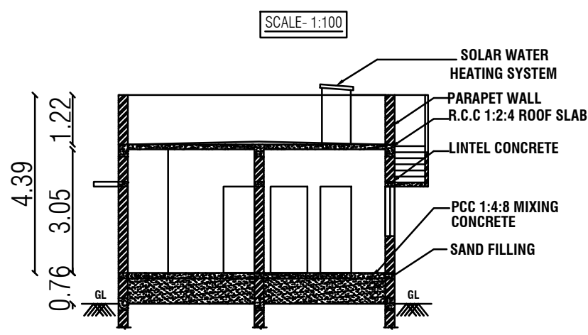
SECTION NO - "AB"
