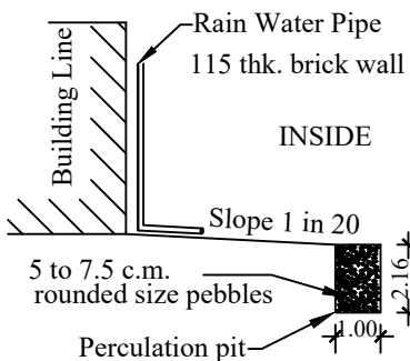
RAIN WATER HARVESTING PERCOLATION PIT
