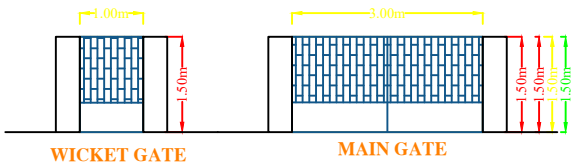
WICKET GATE
