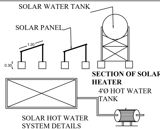
SOLAR HOT WATER SYSTEM DETAILS
