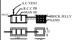
DETAILS OF SEPTIC TANK & DISPERSION TRENCH
