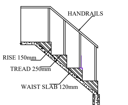
STAIRCASE DETAILS
