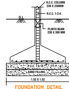
FOUNDATION DETAIL
