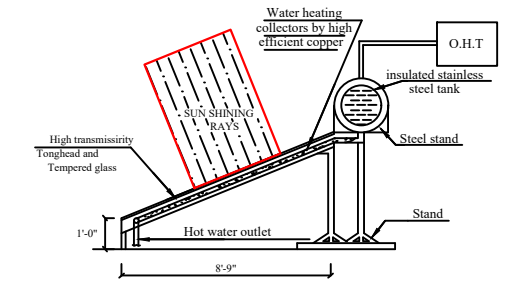
SECTION SOLAR WATER HEATER
