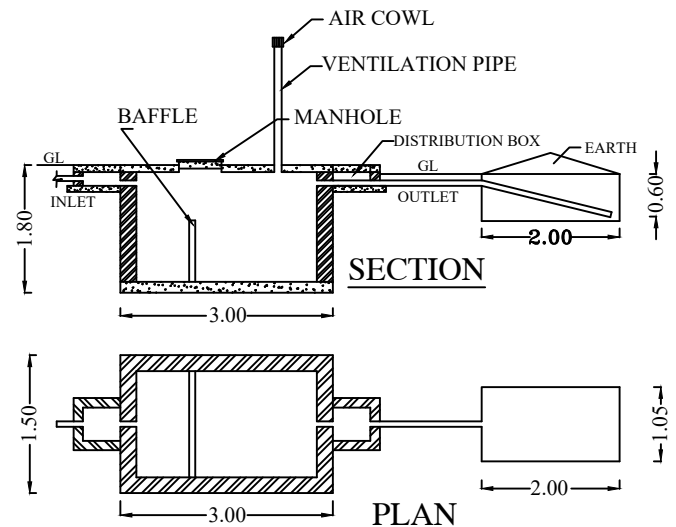
SEPTIC TANK DISPERSION TRENCH
