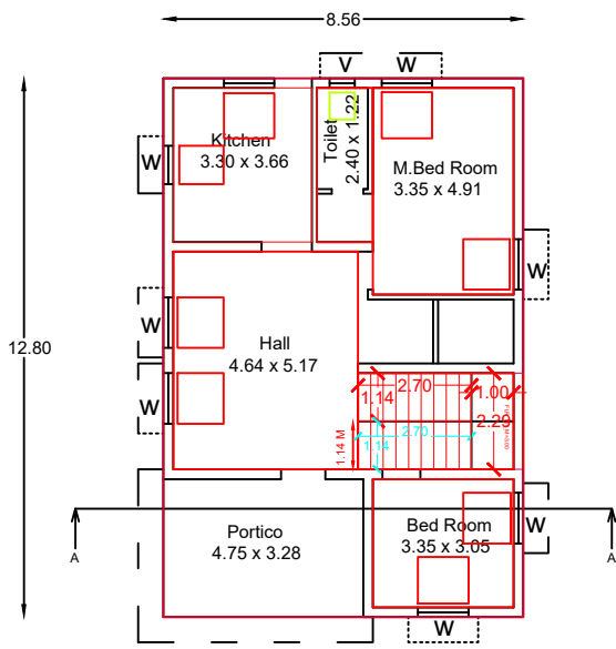
PRO. GROUND FLOOR AREA
