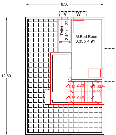
PRO. FIRST FLOOR AREA
