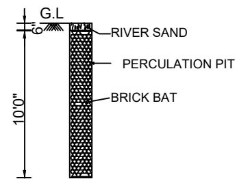
PERCULATION PIT
