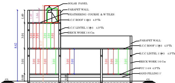
CUT SECTION ON AA
