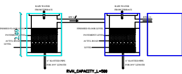
DETAILS OF PERCOLATION PIT
