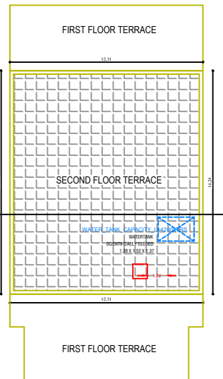
SITE CUM TERRACE FLOOR PLAN
