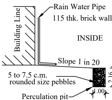
RAIN WATER HARVESTING PERCUSSION PIT
