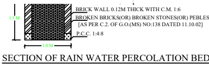
SECTION OF RAIN WATER PERCOLATION BED
