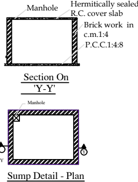
RWH_CAPACITY_L=1000 SUMP_CAPACITY_L=1000LTRS
