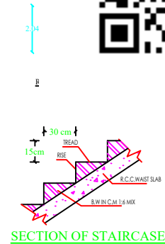
SECTION OF STAIRCASE
