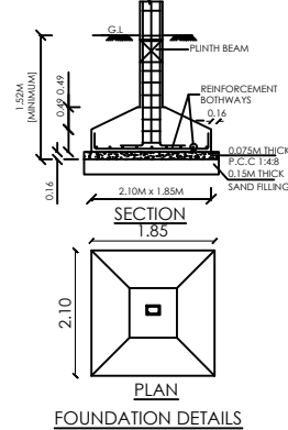
FOUNDATION DETAILS
