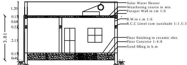
SECTION - "AB "
