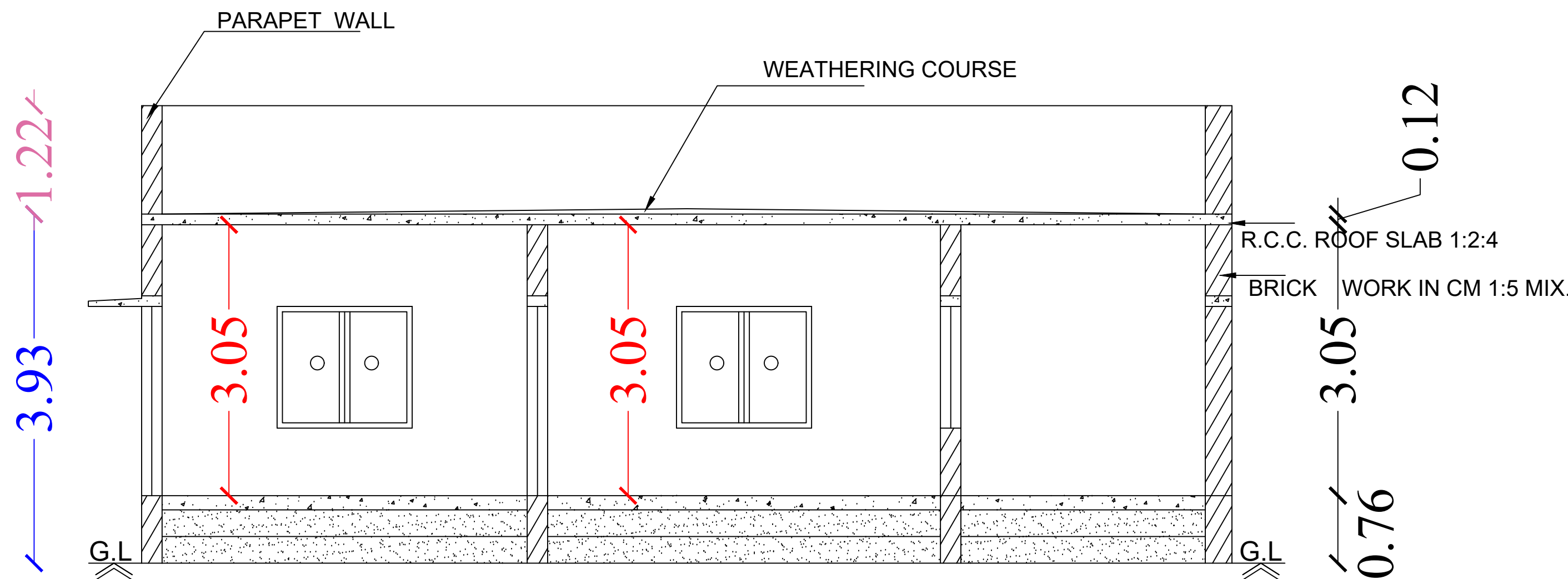
Section on-"AA"
