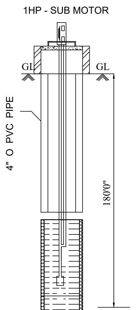
Bore Well Details
