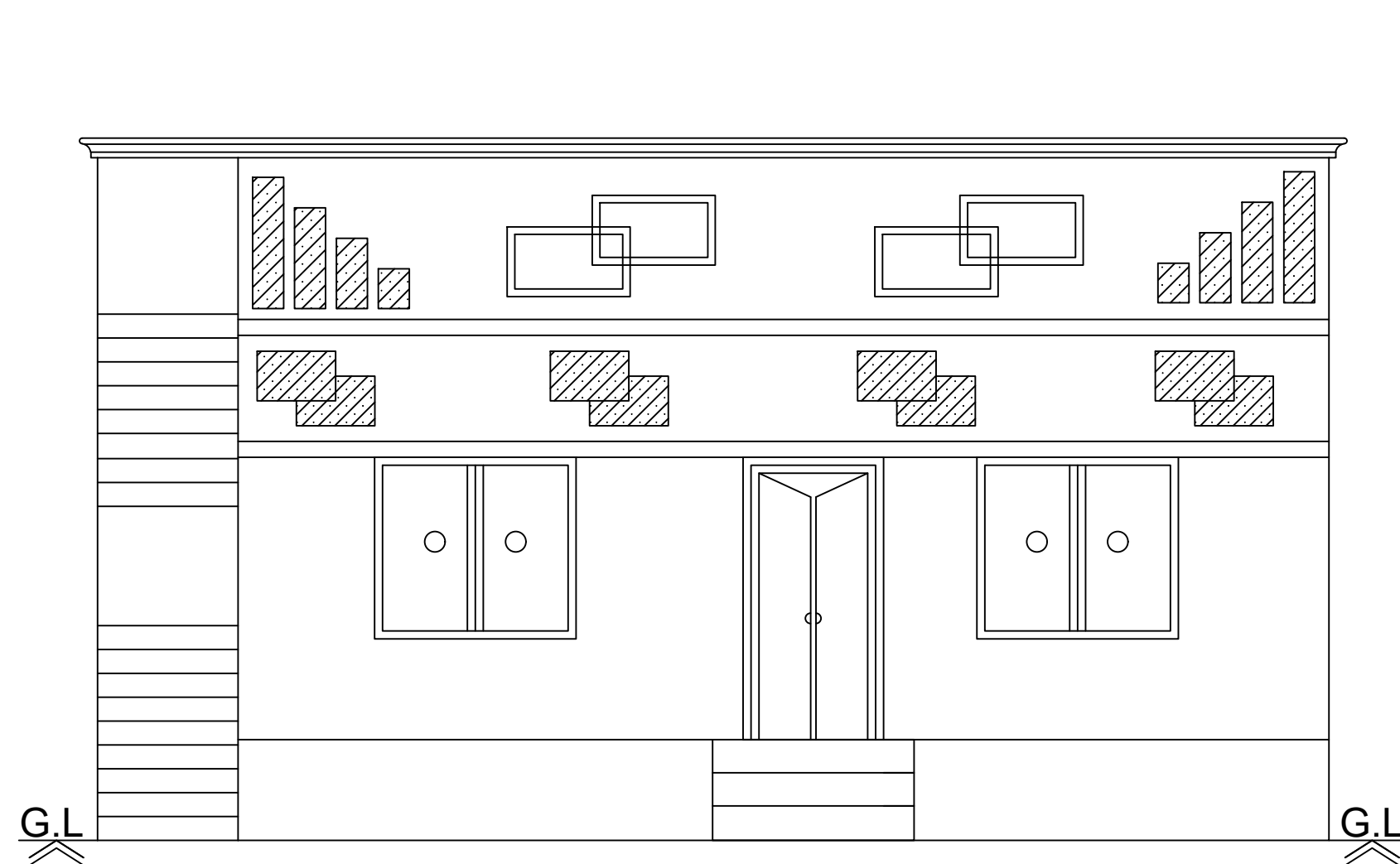
Front Elevation
