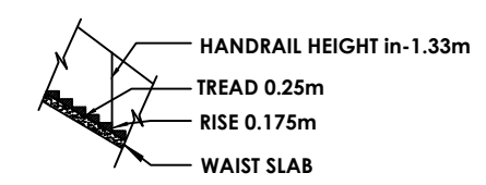
STAIRCASE DETAILS
