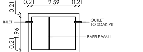
PLAN SEPTIC TANK
