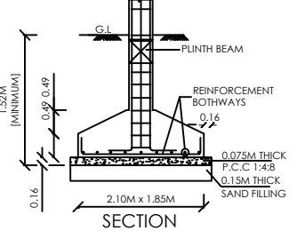
SECTION 1.85
