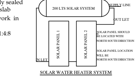
SOLAR WATER HEATER SYSTEM
