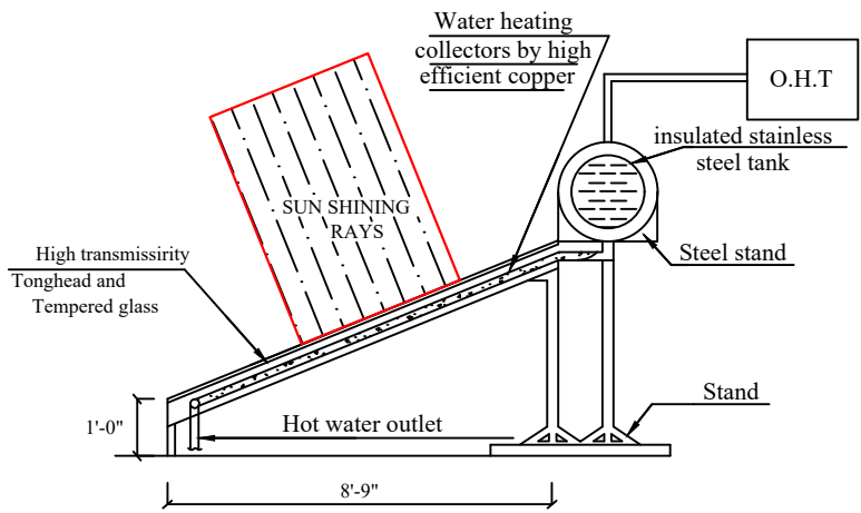
SECTION
