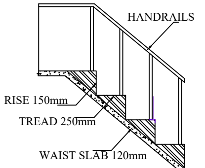
STAIRCASE DETAILS
