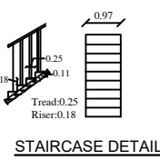
STAIRCASE DETAIL
