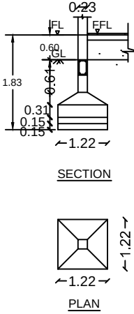
FOUNDATION COLUMN DETAIL
