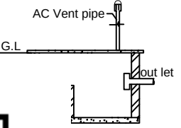
F SEPTIC TANK
