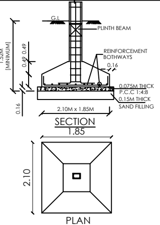
FOUNDATION DETAILS
