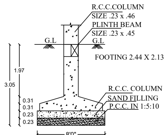
FOUNDATION DETAIL-B
