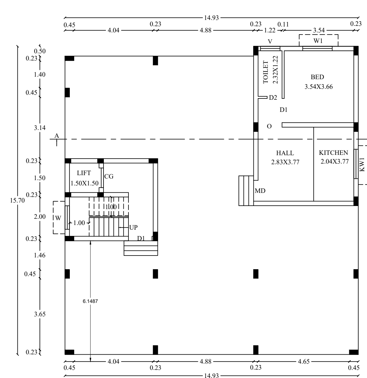
FLOOR PLAN
