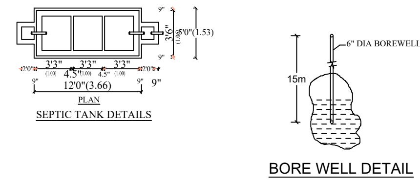
BORE WELL DETAIL
