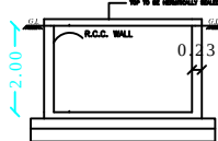
R.C.C WALL SECTION (SAMPLE)
