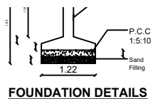
FOUNDATION DETAILS
