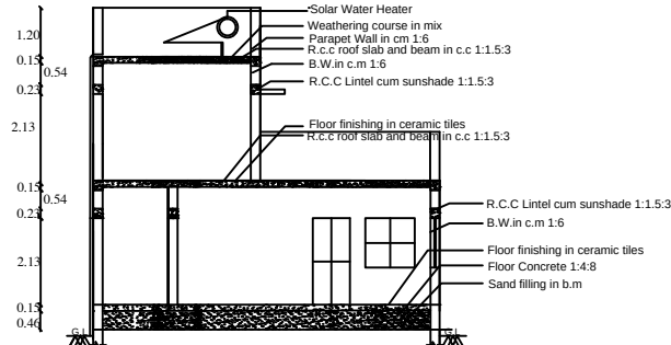
SECTION - "AB - CD "
