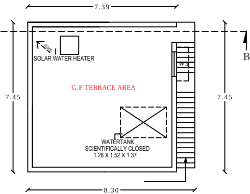
TERRACE FLOOR
