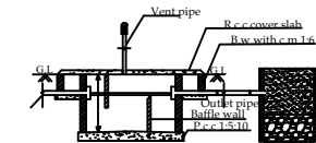
SECTION
