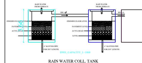
RAIN WATER COLL. TANK
