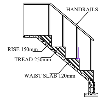
STAIRCASE DETAILS
