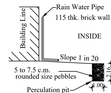
RAIN WATER HARVESTING PERCOLATION PIT
