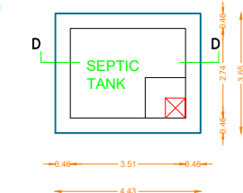
PLAN OF SEPTIC TANK
