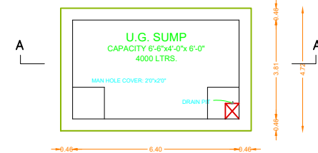
SUMP DETAIL
