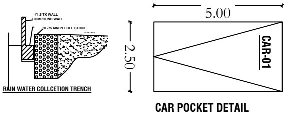
CAR POCKET DETAIL
