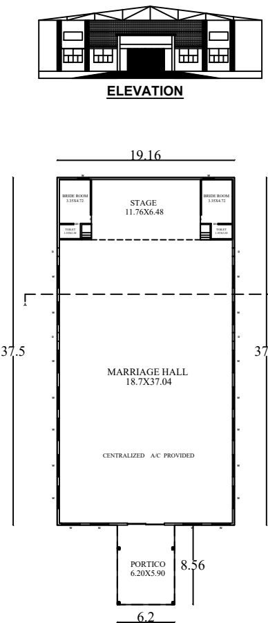
GROUND FLOOR PLAN BLOCK -1
