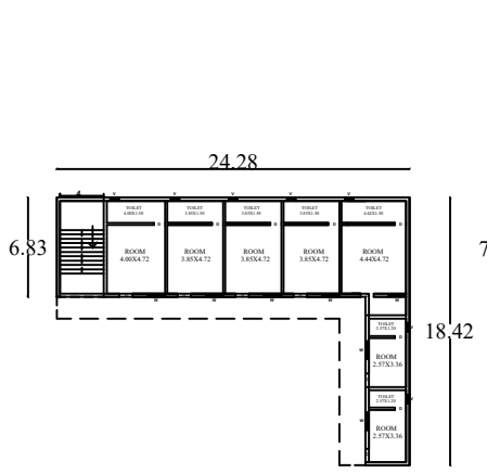
FIRST FLOOR PLAN BLOCK -2
