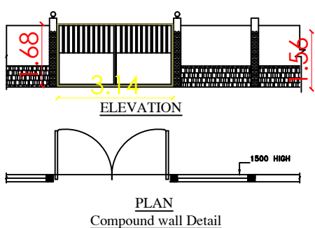
PLAN Compound wall Detail
