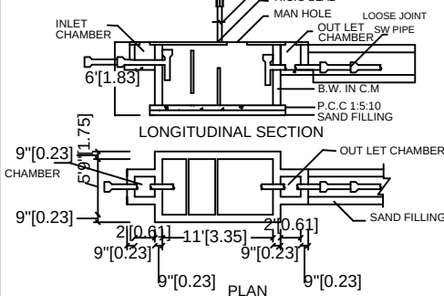
SEPTIC TANK:
