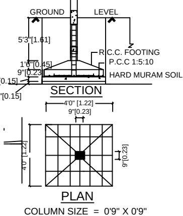
FOUNDATION DETAILS
