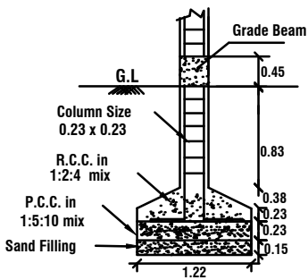
COLUMN DETAILS
