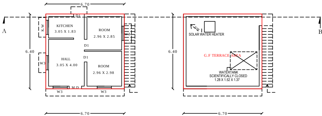
TERRACE FLOOR
