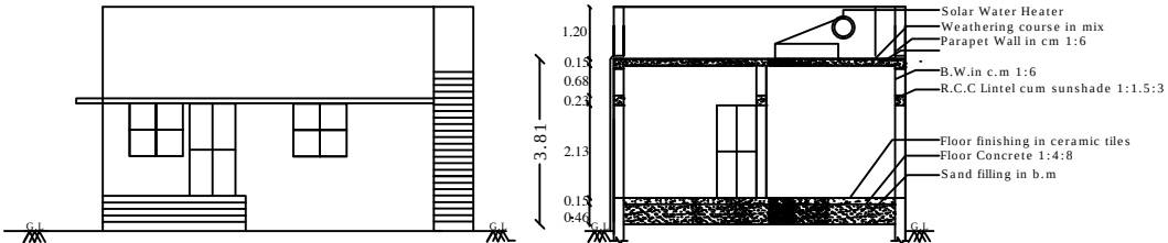
SECTION - "AB "
