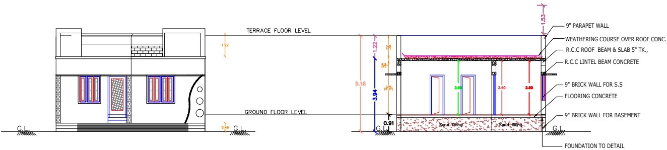
FRONT ELEVATION
