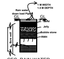
SEC. RAIN WATER HARVEST PIT
