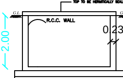
RWH SECTION (SAMPLE) RWH CAPACITY: 15000LTRS
