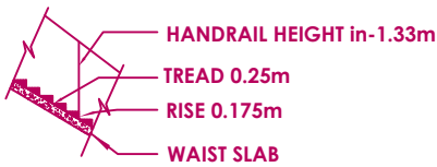
STAIRCASE DETAILS
