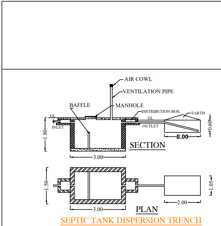
SEPTIC TANK DISPERSION TRENCH
