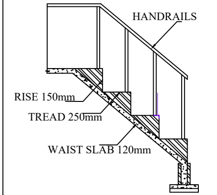
STAIRCASE DETAILS
