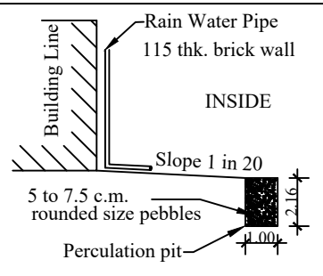
RAIN WATER HARVESTING PERCOLATION PIT
