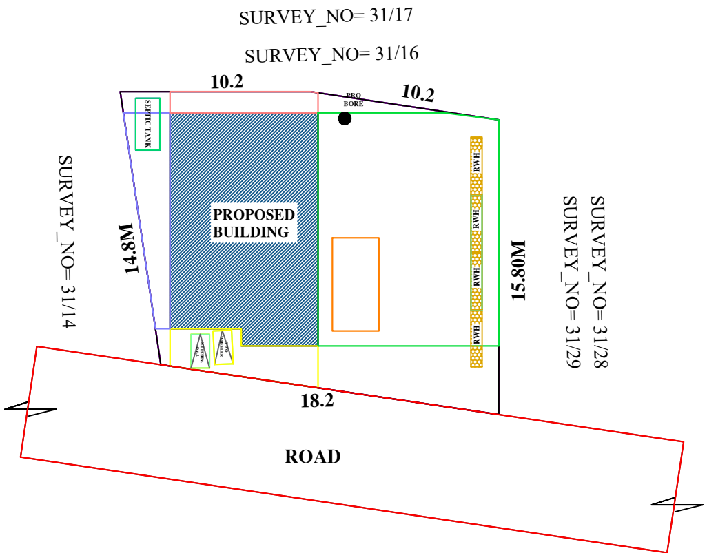
SITE PLAN
