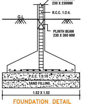
FOUNDATION DETAIL
