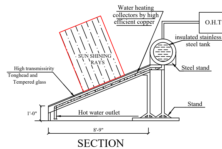
SOLAR WATER HEATER
