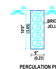
PERCULATION PIT
