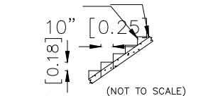
SECTION ON STAIRCASE
