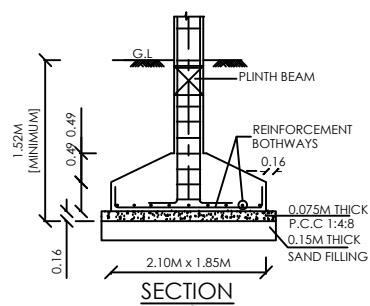
1.85 2.10 PLAN FOUNDATION DETAILS
