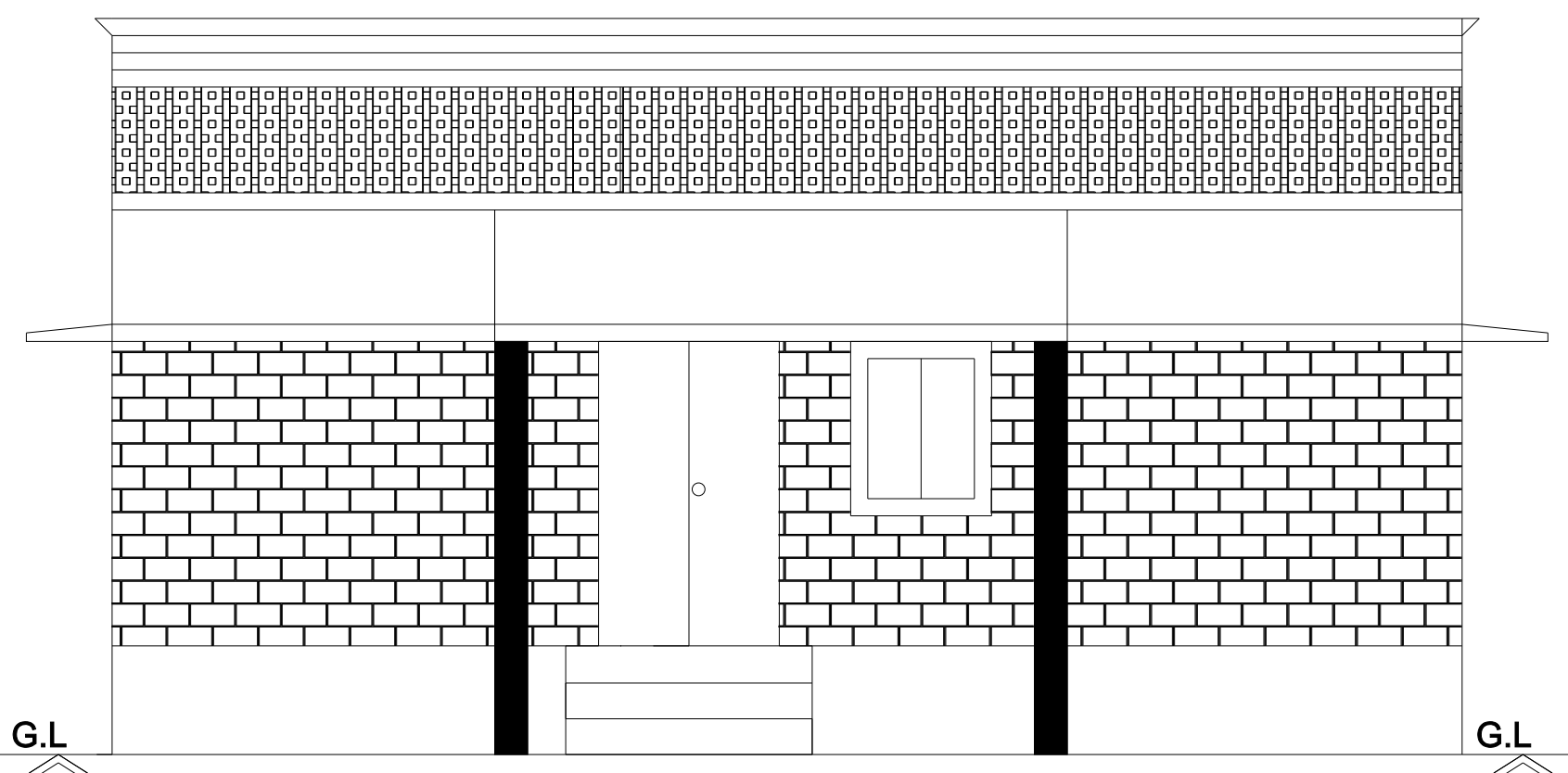
Front Elevation
