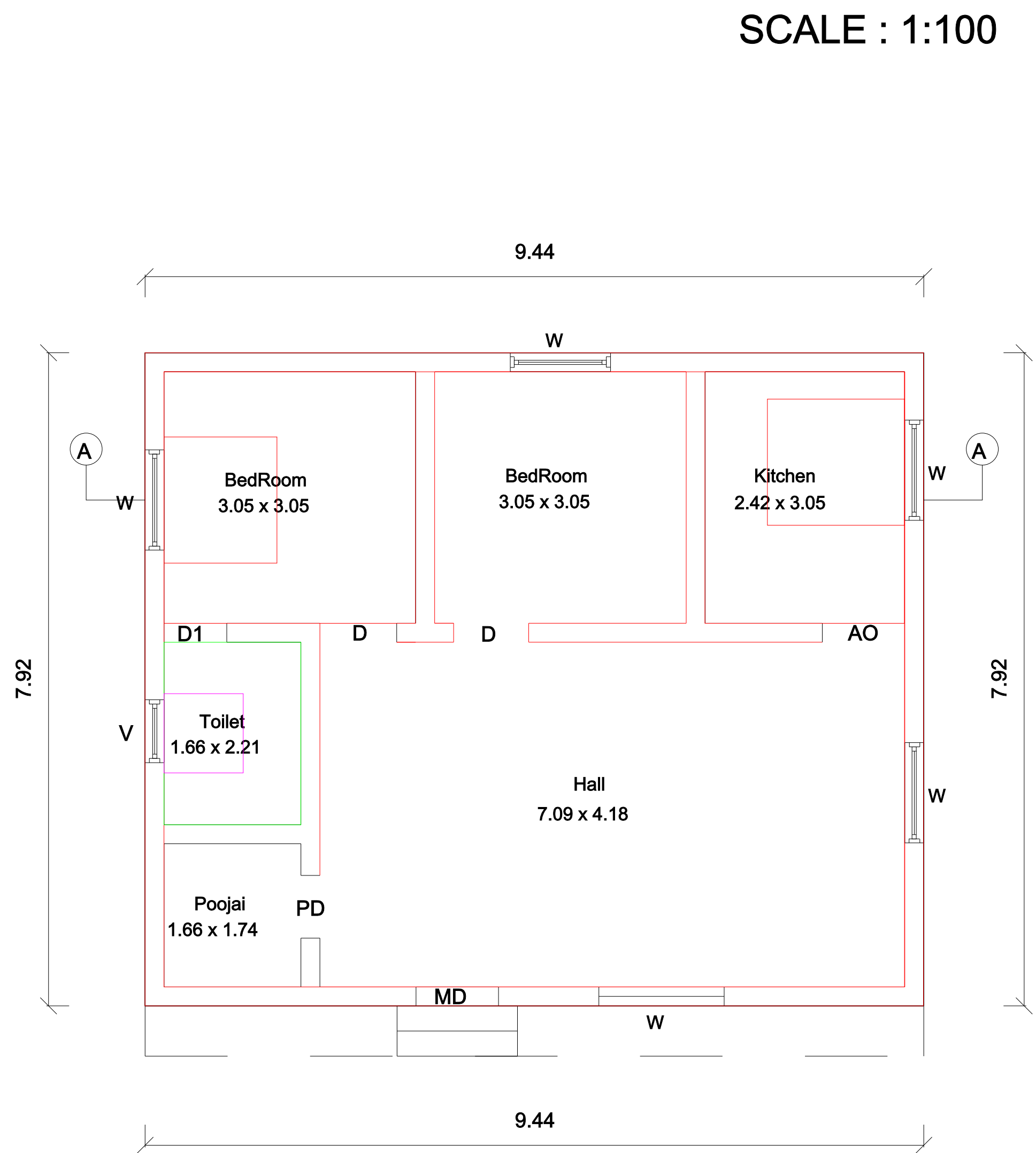
Ground Floor
