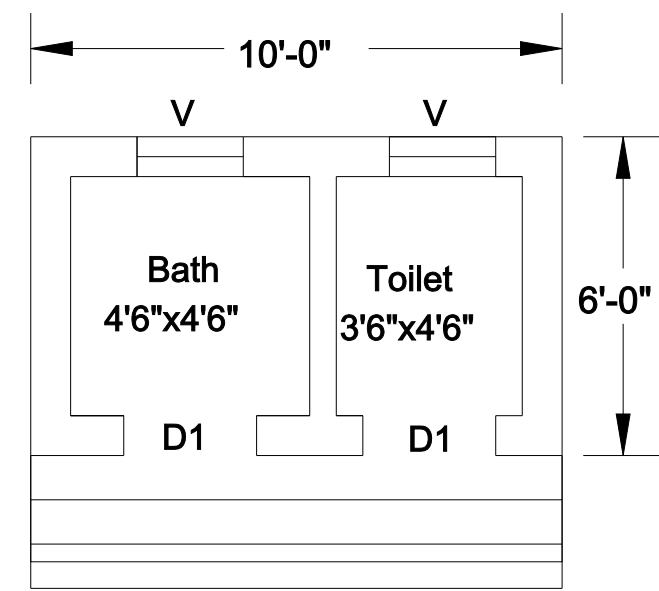
PLAN OF TOILET BLOCK
