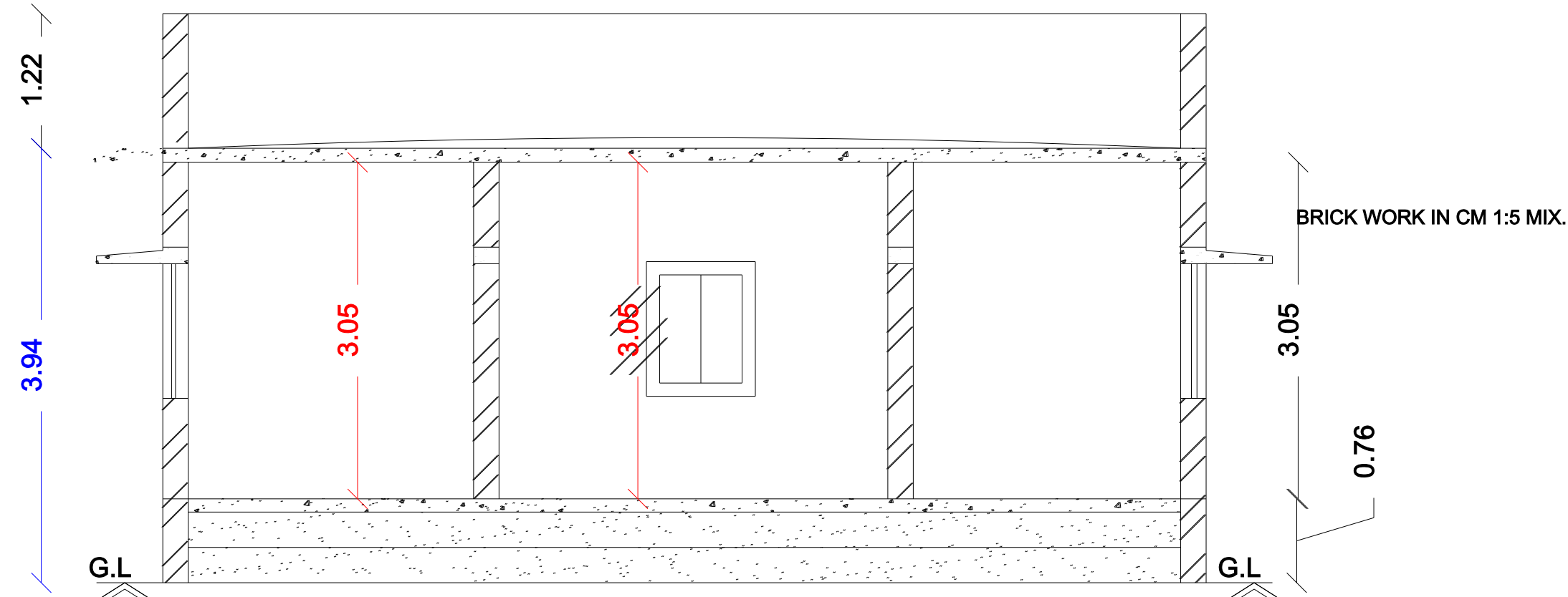
Section on-"AA"
