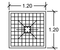
PLAN COLUMN FOOTING DETAILS
