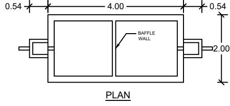
PLAN SEPTIC TANK DETAILS
