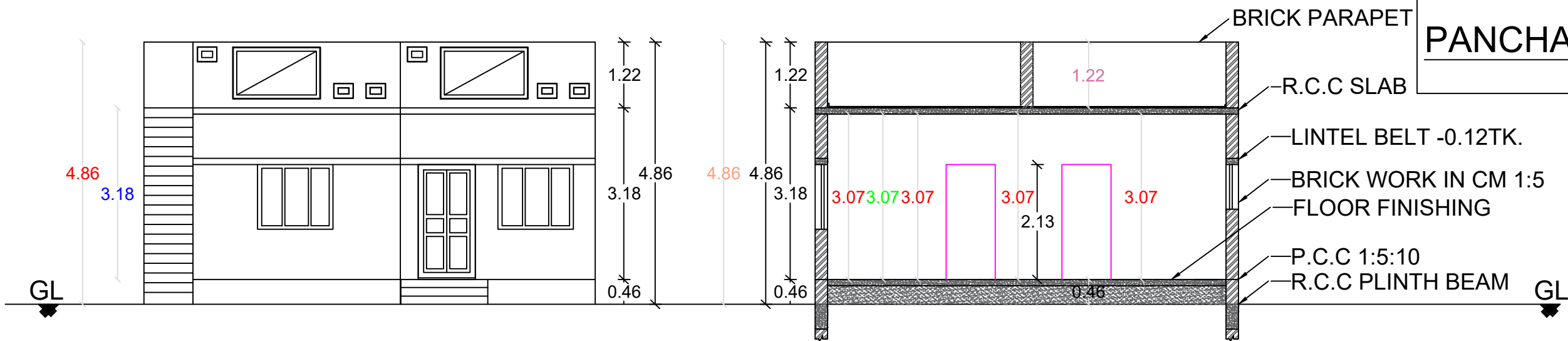
CROSS-SECTION
