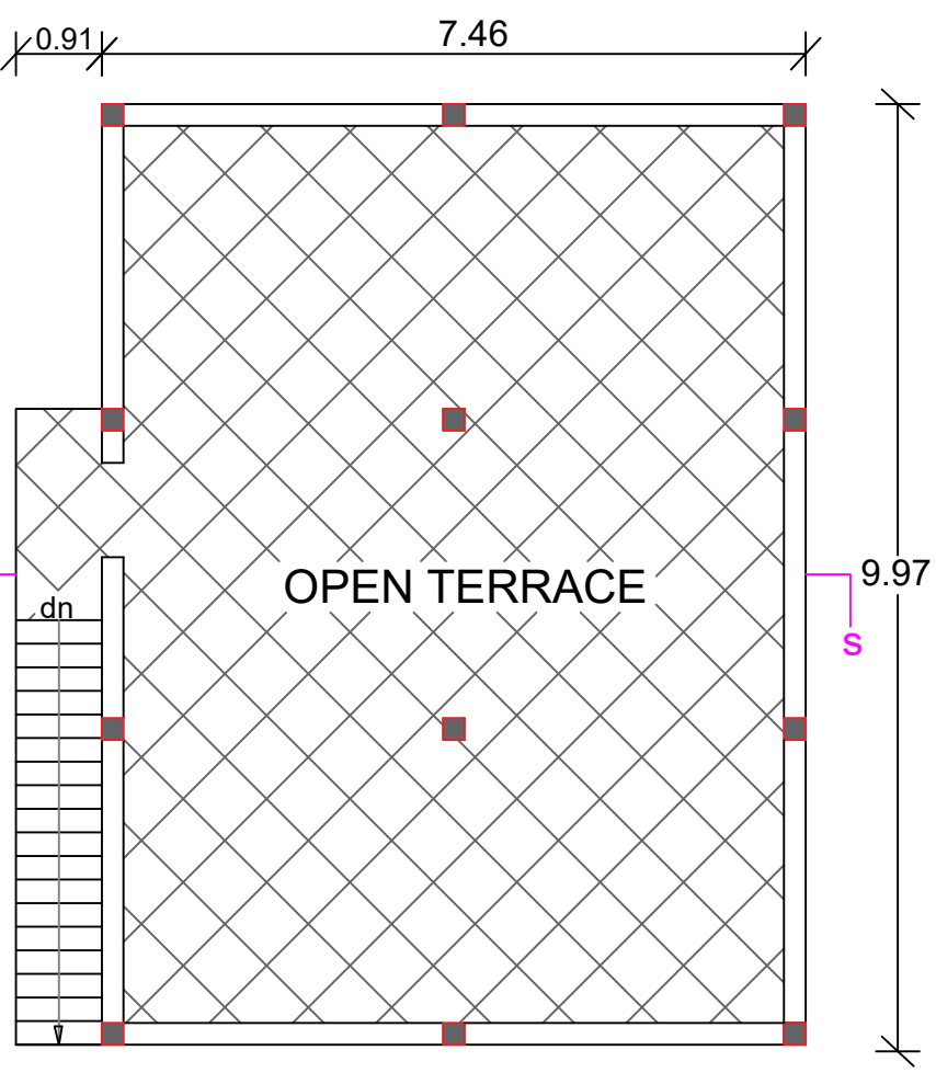
OPEN TERRACE PLAN
