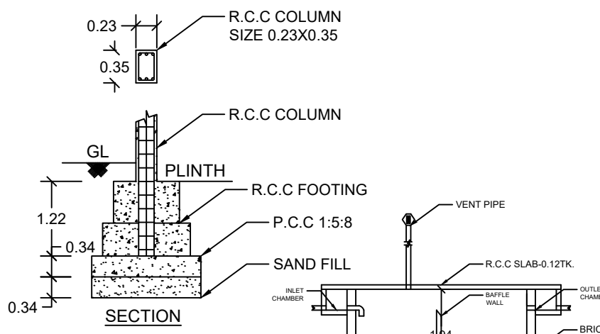
SECTION
