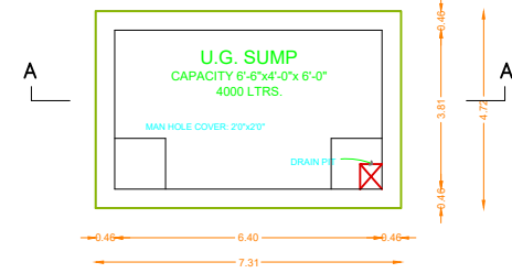
SUMP DETAIL SCALE 1"=4'
