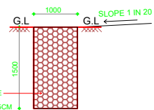
SECTION OF PEBBLE TRENCH SCALE : 1 : 100
