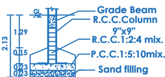
COLUMN DETAILS
