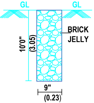
PERCOLATION PIT
