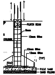
FOUNDATION DETAILS SCALE : 1:50.
