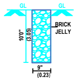
PERCULATION PIT
