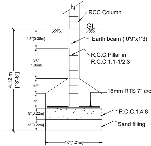
FOUNDATION DETAILS
