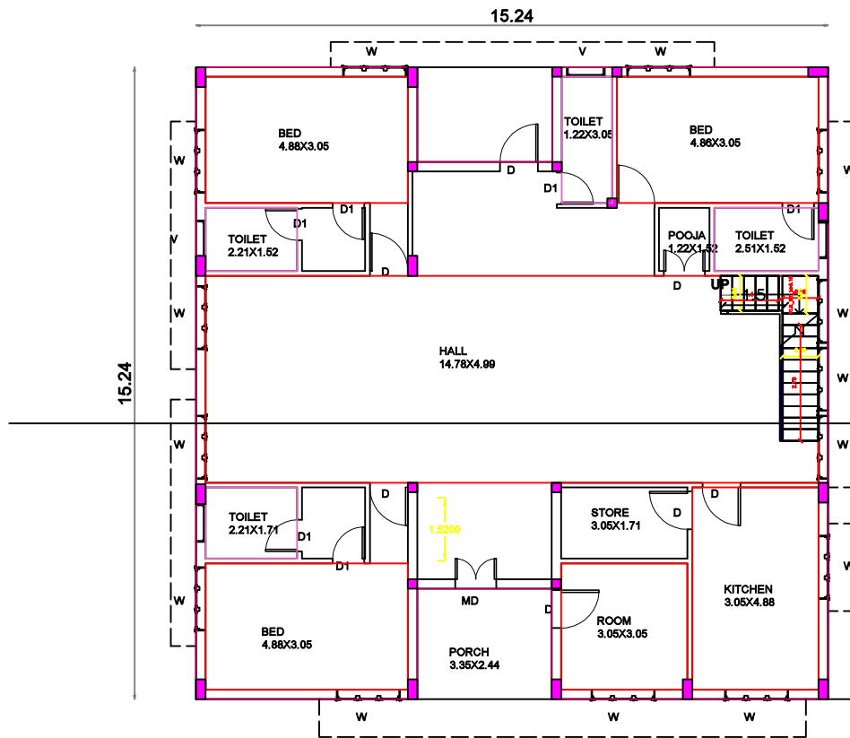
PROPOSED SITE CUM GROUND FLOOR PLAN
